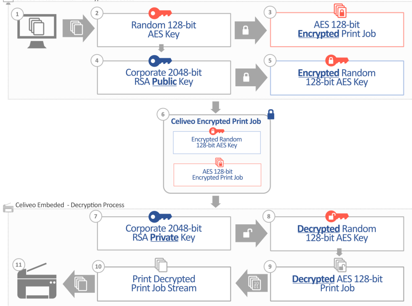
Celiveo Virtual Printer - Encryption Process
